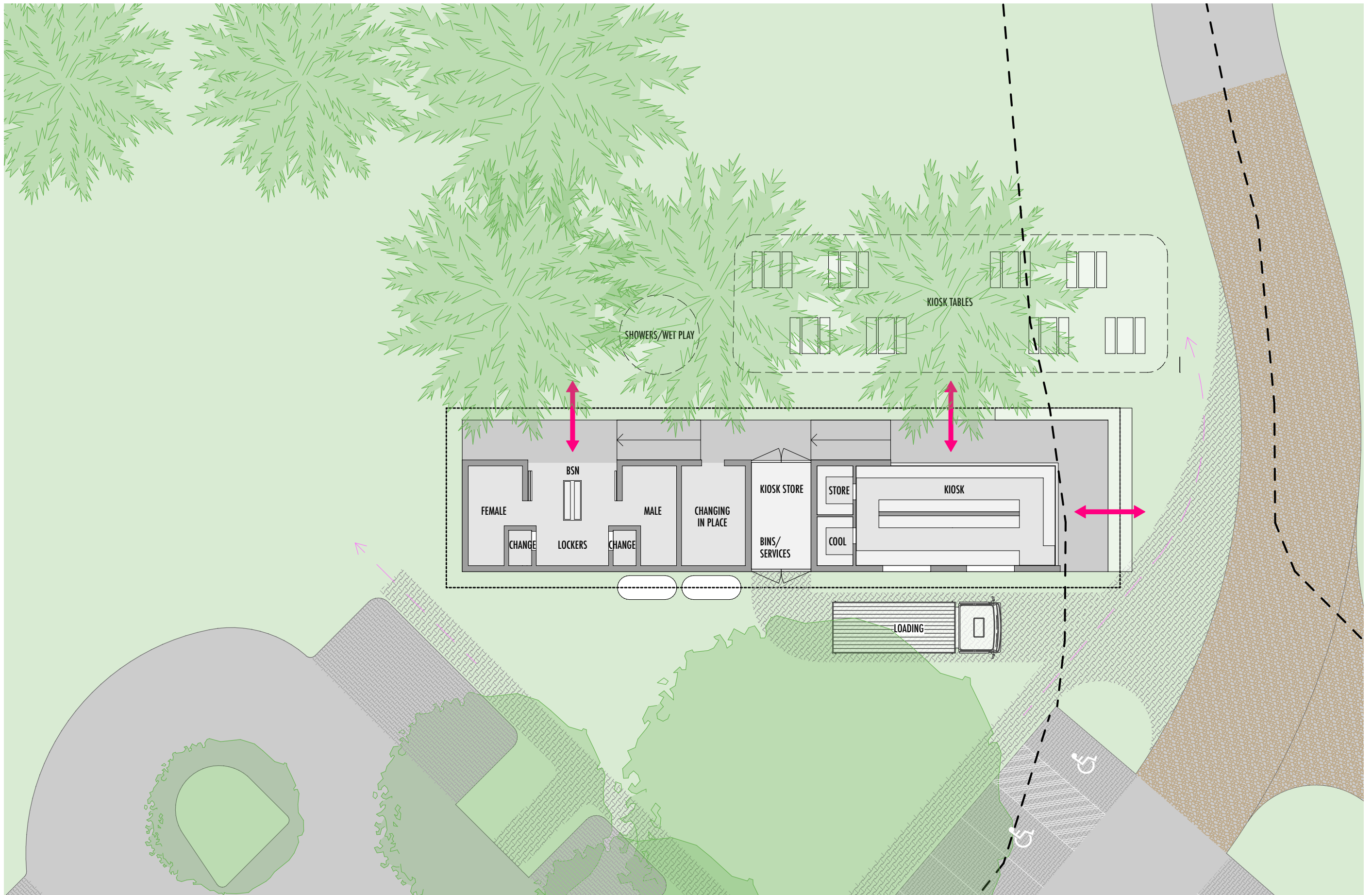
HORSESHOE BAY AMENITIES & KIOSK LAYOUT
